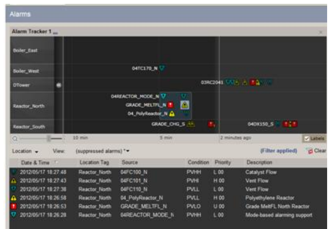
Figure 3 - Alarm Tracker
