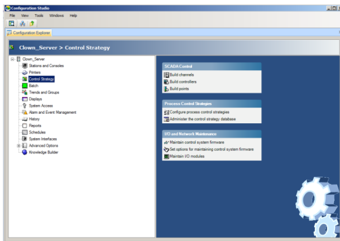
Figure 7 – Configuration Studio
